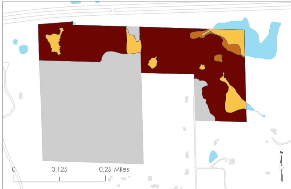
Floristic Quality Index
