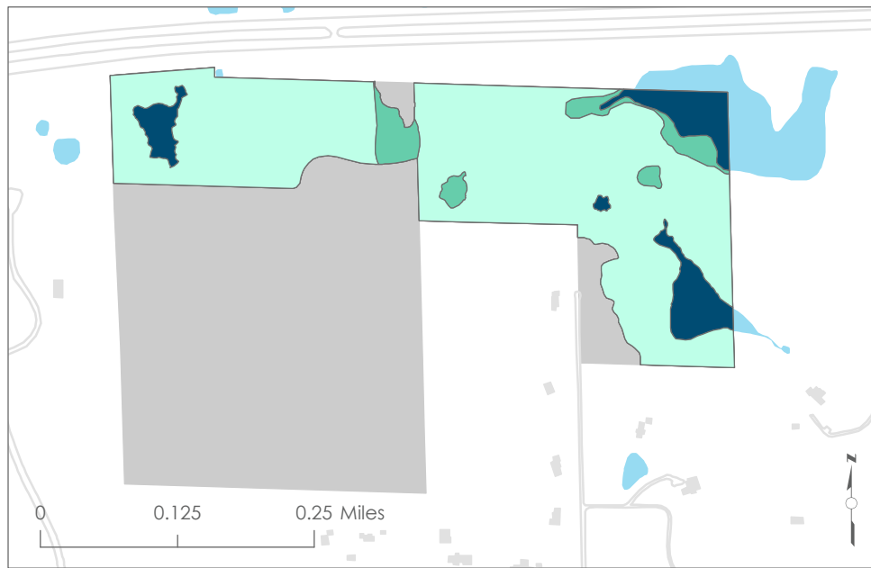
Mean Coefficient of Wetness
