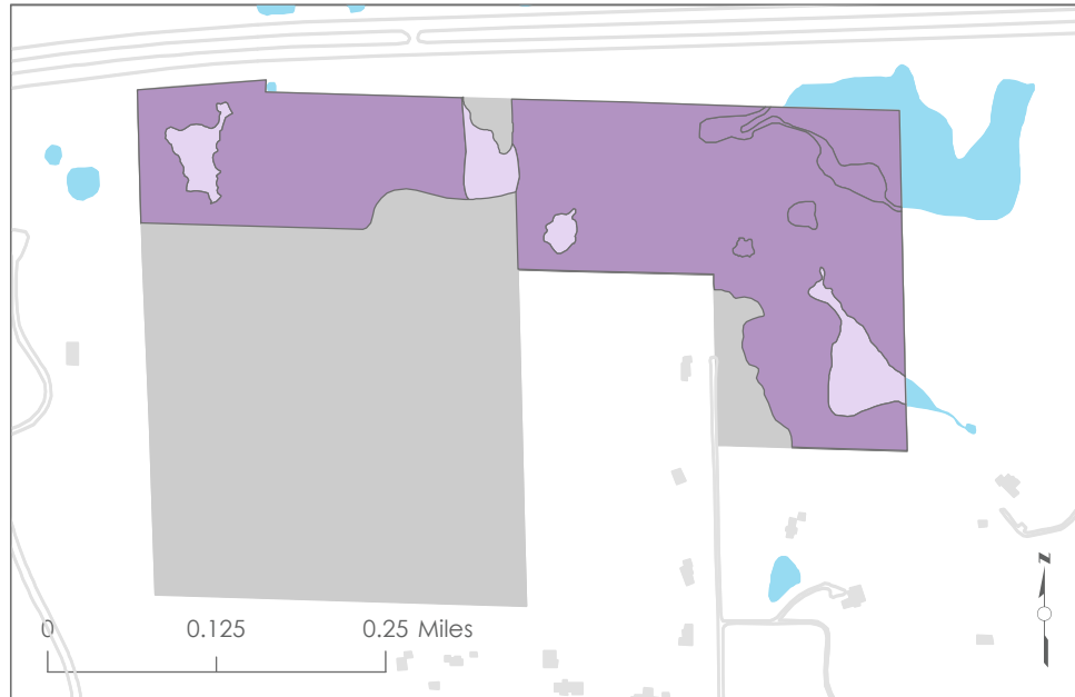
Mean Coefficient of Conservatism
